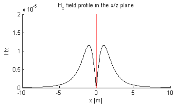
Fig. 13 vertical dipole
