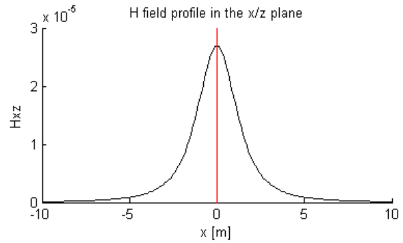
Fig. 12 vertical dipole
